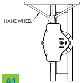
STANDARD HANDWHEEL ORIENTATION
