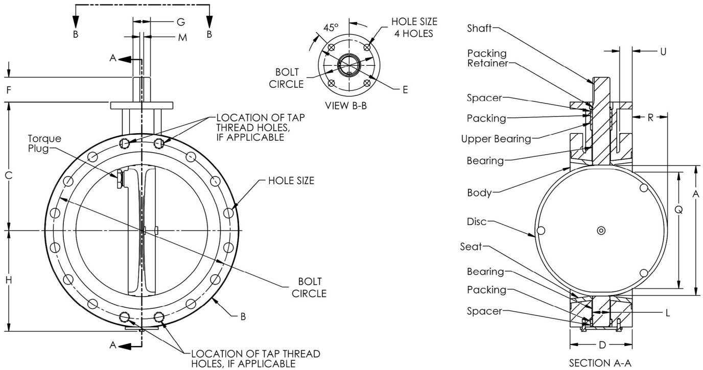
K-Flo Model 507 250B (Flanged x Flanged***)
